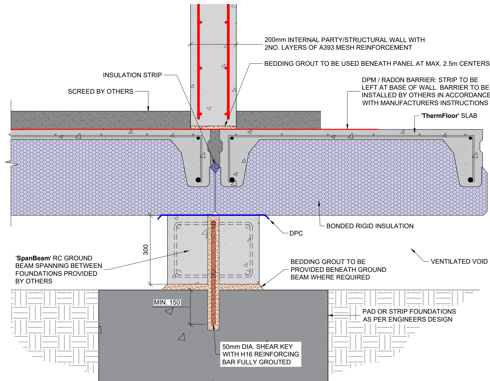
TYPICAL SECTION THROUGH PARTY WALL/INTERNAL STRUCTURAL WALL SUPPORTS - DETAIL A SCALE 1:10
