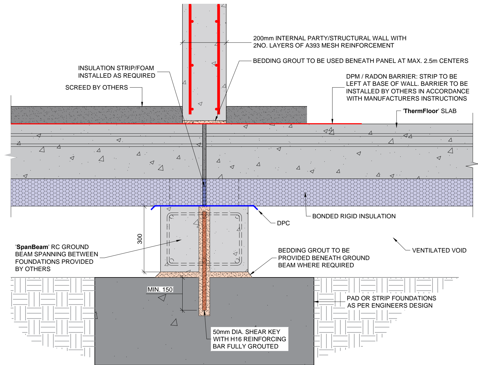
TYPICAL SECTION THROUGH PARTY WALL/INTERNAL STRUCTURAL WALL SUPPORTS - DETAIL B SCALE 1:10
