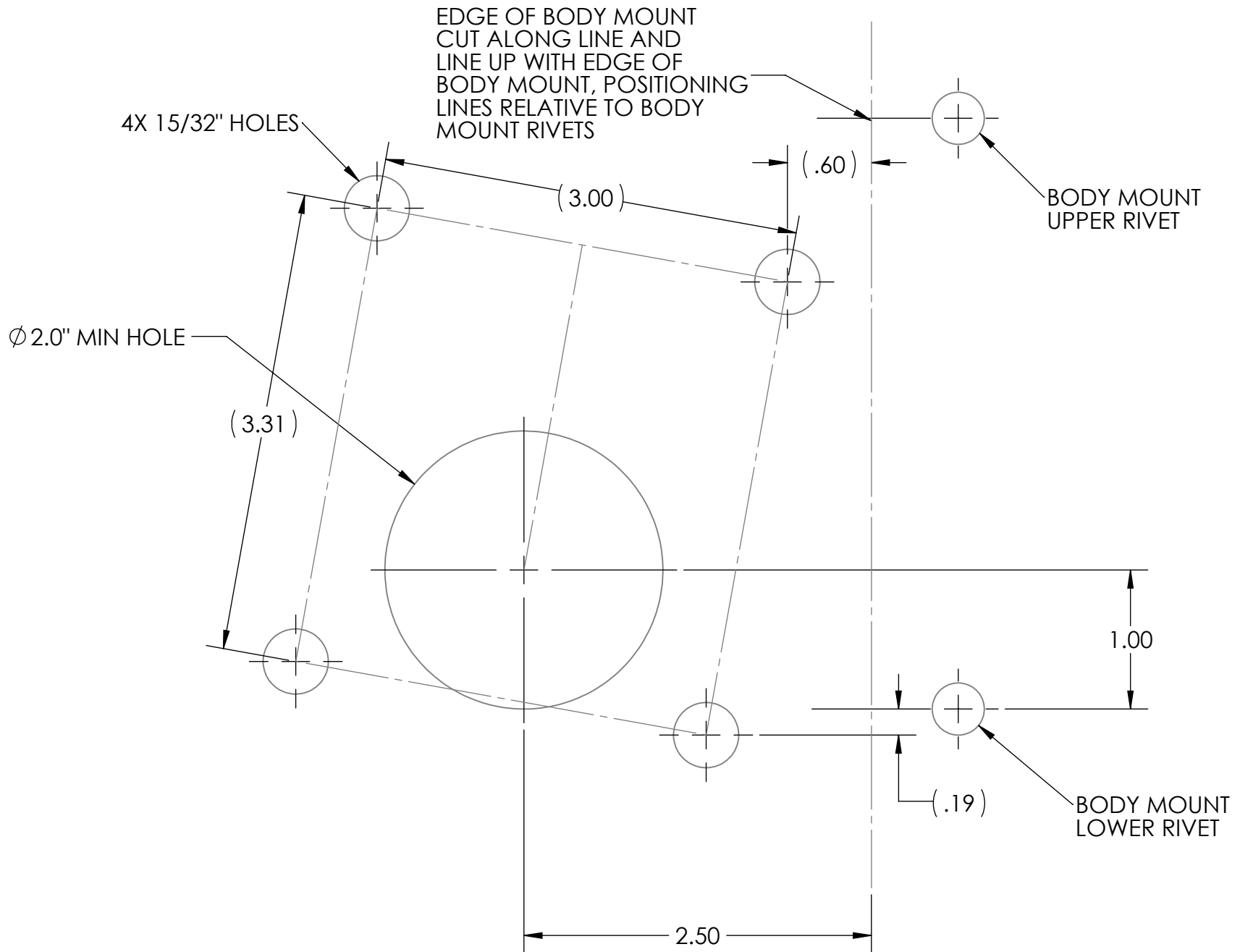
FRONT UPPER SPRING BUSHING MOUNT DRIVERS SIDE TEMPLATE -PRINT ON 8.5" X 11" AT 100% SCALE
