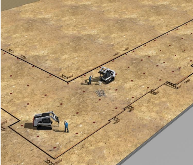
Multiple Helical Piers can be installed simultaneously reducing construction time
