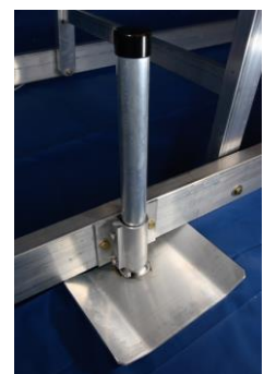
Adjustable Legs
