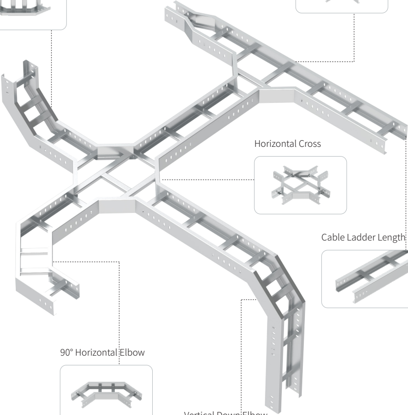
Vertical Down Elbow
