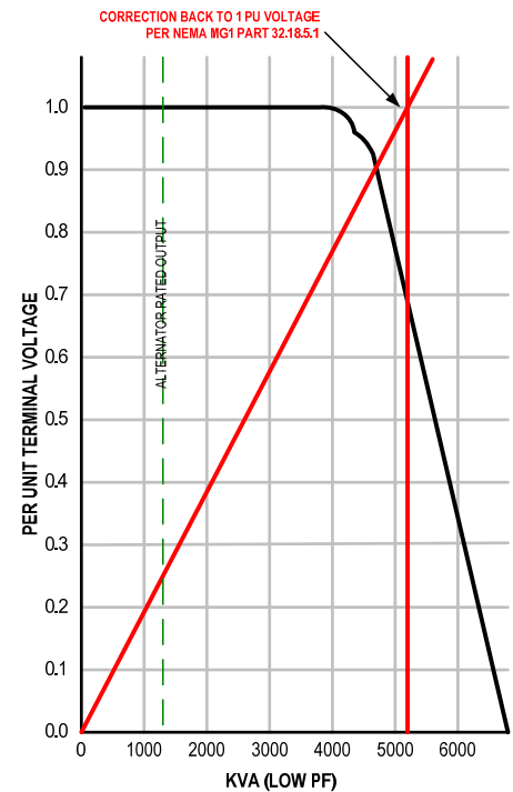
Figure 6: Field Forcing Capability Curve for a 1250kVA generator set.
