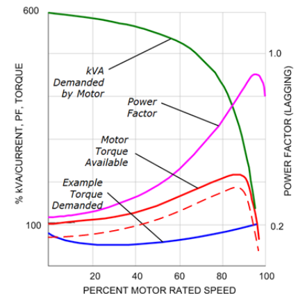
Figure 3: Dashed red line indicates available torque with 90% of nominal voltage.
