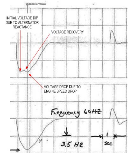
Figure 4: Generator set performance on application of a block load. Note that voltage begins to recover by drops again due to engine speed drop.
