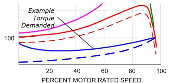
Figure 5: Torque demand of different motors based on the nature of their loads. Dashed blue line shows torque demand of a low inertia motor load.
