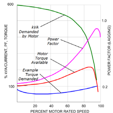
Figure 1: Typical motor starting curve
