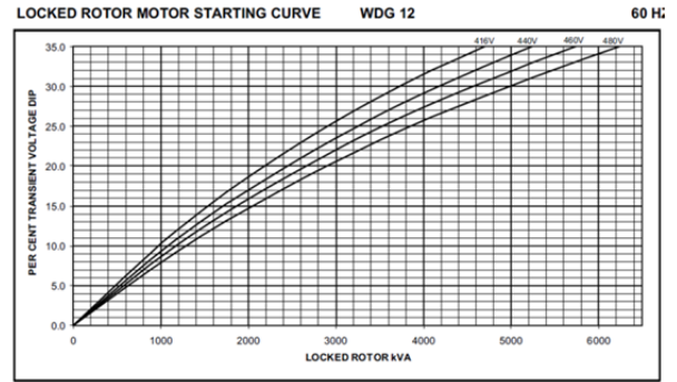
Figure 2: Typical voltage dip (aka "motor starting") curve.
