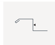
Z-Flashing TN-06
