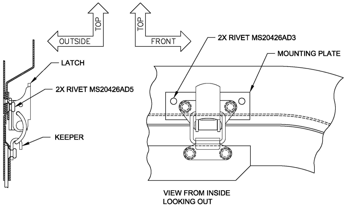
Latch and Handle Installation Figure 7
