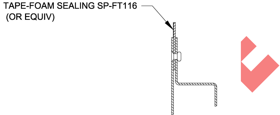
Retainer Seal Installation Figure 6
