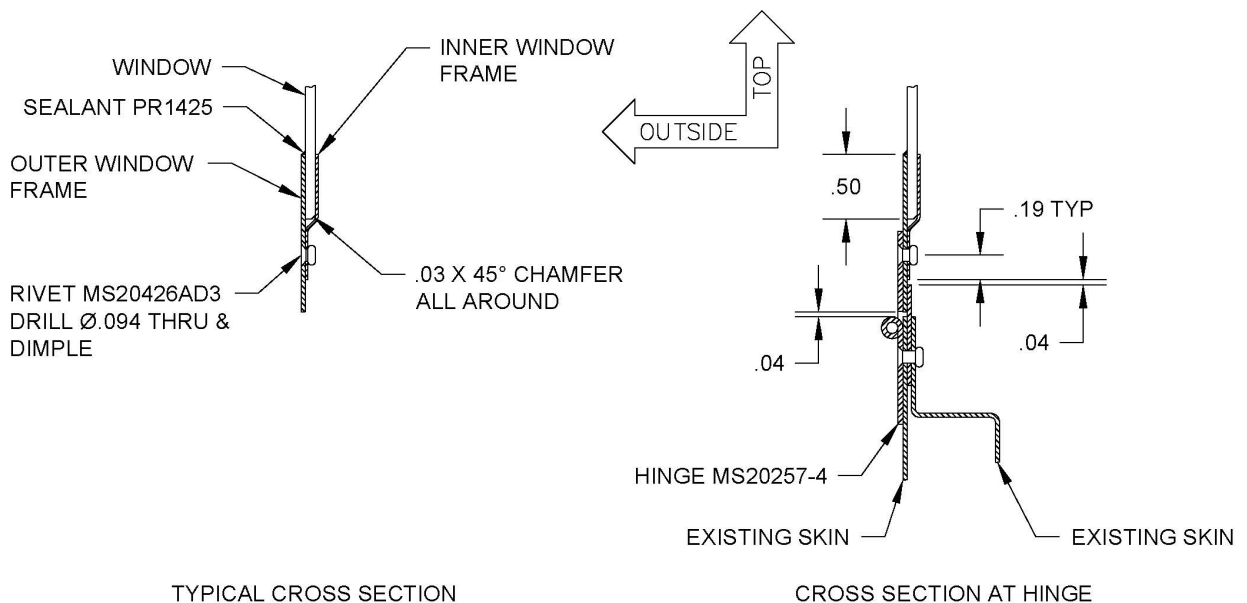
Window Assembly Figure 4
