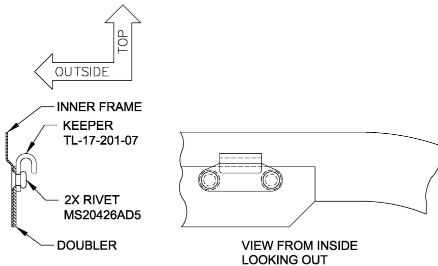
Keeper Installation Figure 3
