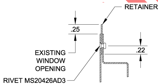
VIEW E Inner and Outer Window Frame & Window Retainer Fabrication Figure 1 (Cont)
