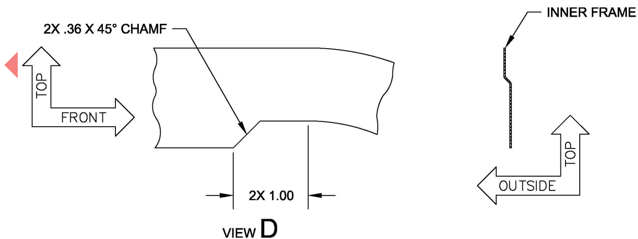
Inner and Outer Window Frame & Window Retainer Fabrication Figure 1
