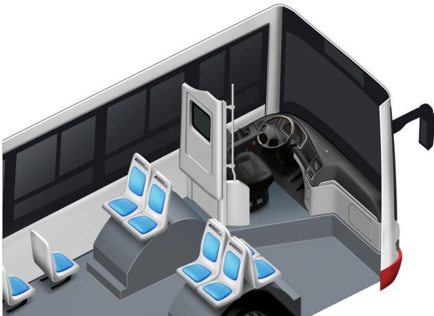
Semi-closed cab design
