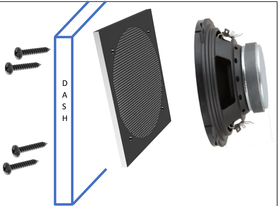
1968 to 1977 Speaker Grille installation
