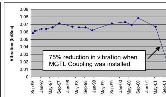
Vertical Axis Vibration Measurement
