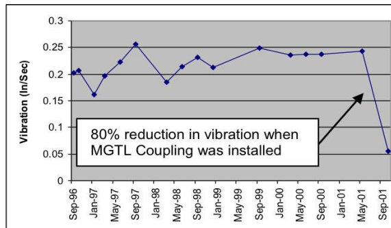
Horizontal Axis Vibration Measurement
