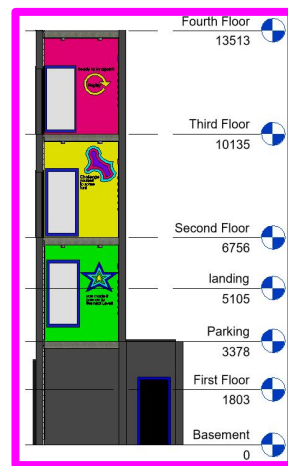
South Section
