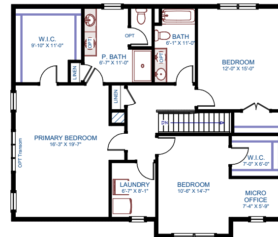
SECOND FLOOR (Standard)
