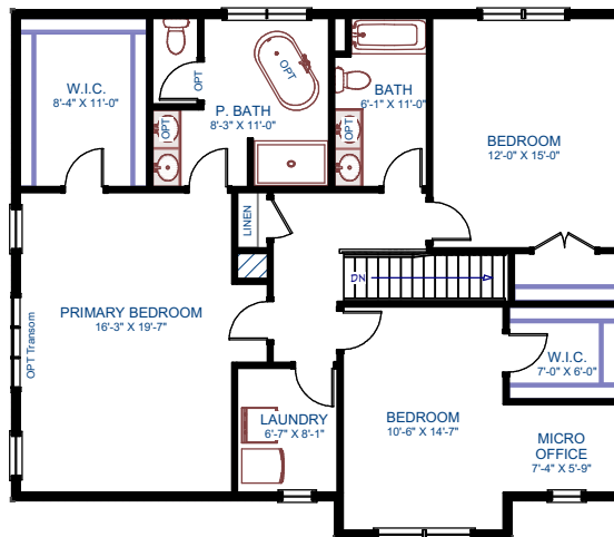
SECOND FLOOR (Deluxe Bathroom)
