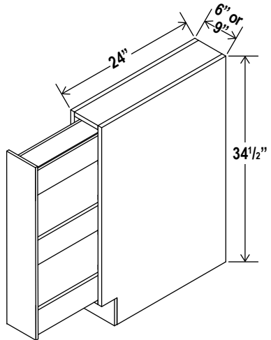
Spice Pull Base Cabinet
