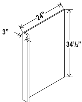
Dishwasher Return Panel
