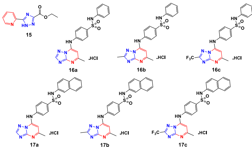
Figure 9. Pyridine or pyrimidine containing antimalarial 1,2,4-triazoles.
