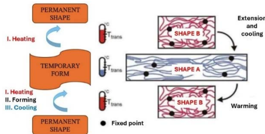
Figure 5. a. Programming of shape memory polymer with temperature b. Molecular mechanism of shape memory effect affected by temperature (Boyacıoğlu, 2016; Behl et al., 2007).
