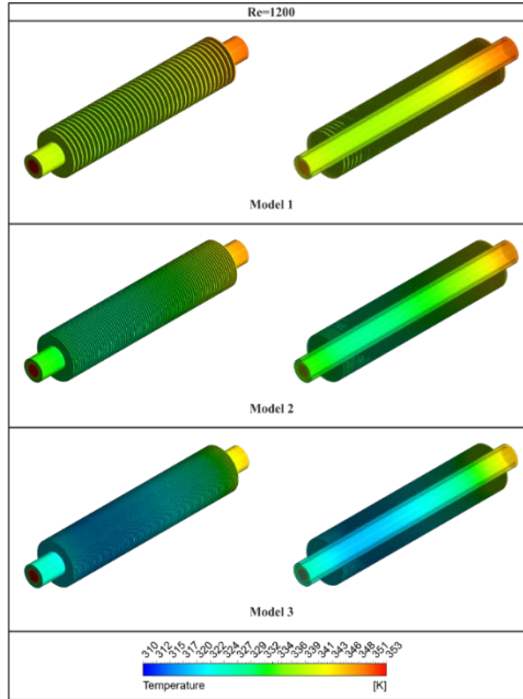
Figure 6. Temperature Distributions for Re=1200
