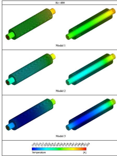
Figure 4. Temperature Distributions for Re=400
