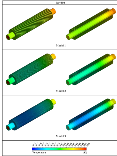
Figure 5. Temperature Distributions for Re=800
