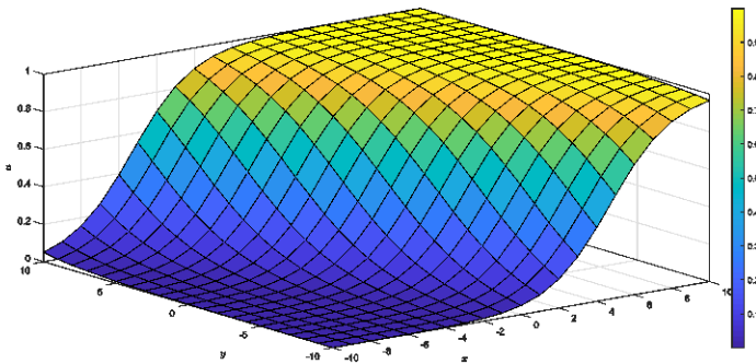
Figure 2. Numerical solution u(x, y, T) as a 3D surface at T = 1 , showing the front connecting the two rest states u = 0 and u = 1 .
