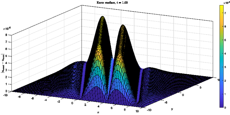
Figure 4. Error surface |u_{\text{exact}} - u_{\text{numerical}}| at T = 1 .
