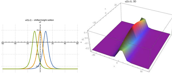
Figure 2. u_2(x, t) for \alpha = 1, \beta = 1.5, \gamma = 1, l = 0.5, m = -0.5 : (a) 2D profile at several t , showing a bright soliton on a nonzero background; (b) 3D surface.
