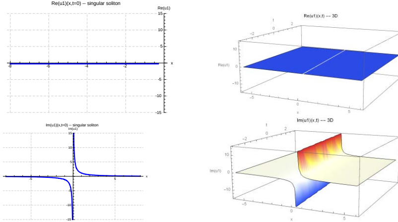
Figure 1. u_1(x, t) for \alpha = 1, \beta = 1.5, \gamma = 1, l = m = 0.5 : (a) \operatorname{Re}(u_1) , constant; (b) \operatorname{Re}(u_1) , 3D flat plane; (c) \operatorname{Im}(u_1) at t = 0 , singular soliton; (d) \operatorname{Im}(u_1)(x, t) , 3D.
