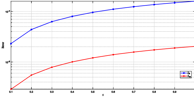
Figure 3. L_2 and L_\infty error norms as functions of t , for N_x = N_y = 160 , \Delta t = 0.003125 (log scale).
