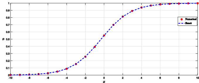
Figure 1. Numerical (circles) and exact (dashed) solution along the cross-section y = y_{\text{mid}} at T = 1 , for N_x = N_y = 160 , \Delta t = 0.003125 .
