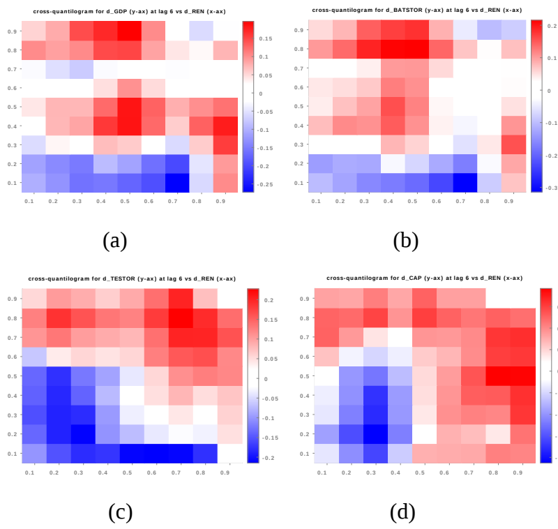
Fig. 3. CQ results for REN at 6 Lags
