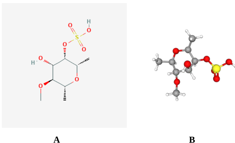
Figure 1. A) 2D B) 3D structures of fucoidan (PubChem n.d)
