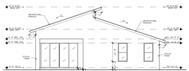
REAR ELEVATION
