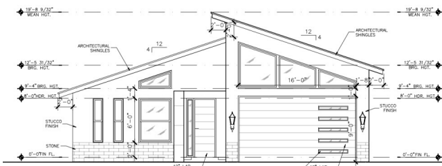
FRONT ELEVATION
