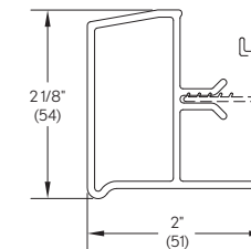
Sill Casing
