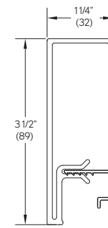
Flat Casing
