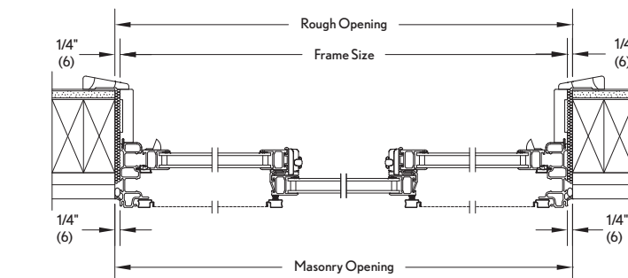
Triple Sash XOX Operator Jamb
