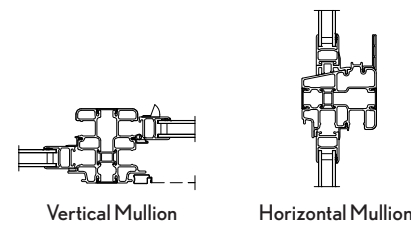
Vertical Mullion
