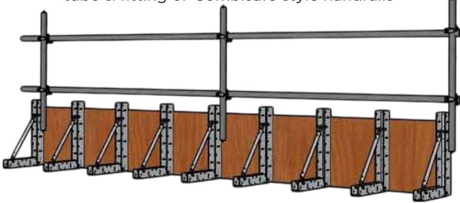
Slab edge with handrail, ability to attach tube & fitting or Combisafe style handrails
