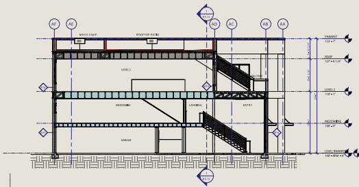
1 BUILDING A - BUILDING SECTION A3.11 1/8" = 1'-0"
