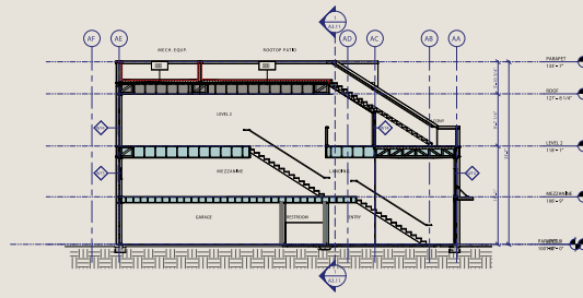
2 BUILDING A - BUILDING SECTION A3.11 1/8" = 1'-0"
