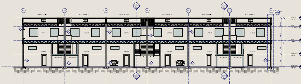
3 BUILDING A - BUILDING SECTION A3.11 1/8" = 1'-0"
