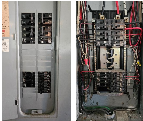
Circuit panel / Copper branch wiring
