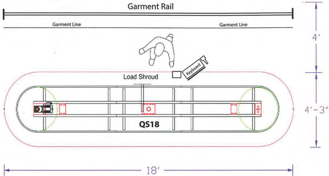
QS18 Typical Layout
