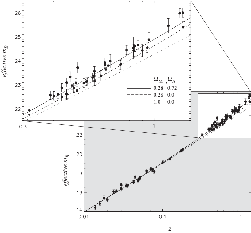
Fig. 11.6. The magnitudes m_B of supernovae of type Ia selected for exhibiting low extinction within their parent galaxies, and plotted against their red shifts z . The magnitudes m_B take red shift into account and correspond to the blue light emitted in the rest-frame of the supernova. The implications of the three curves marked by different values of the symbols \Omega_M and \Omega_\Lambda are discussed below, in Section 11:12. The data were culled from surveys of both nearby and distant supernovae published by different groups in five separate studies. Courtesy of Saul Perlmutter (Pe05).
