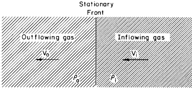
Fig. 9.4. Conditions on the two sides of a shock or ionization front.
