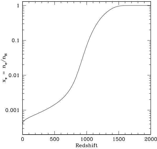
Fig. 13.1. The ratio of electrons to hydrogen atoms as a function of red shift for the assumed parameters \Omega_T = 1.0 , T_0 = 2.725\text{K} , \Omega_B = 0.04 , \Omega_A = 0.73 , a helium abundance by mass, Y = 0.24 , and a Hubble constant H_0 = 70 \text{ km s}^{-1} \text{ Mpc}^{-1} . Courtesy of Sara Seager, who provided this updated version of an earlier plot by Seager, Sasselov, and Scott (Se99).
