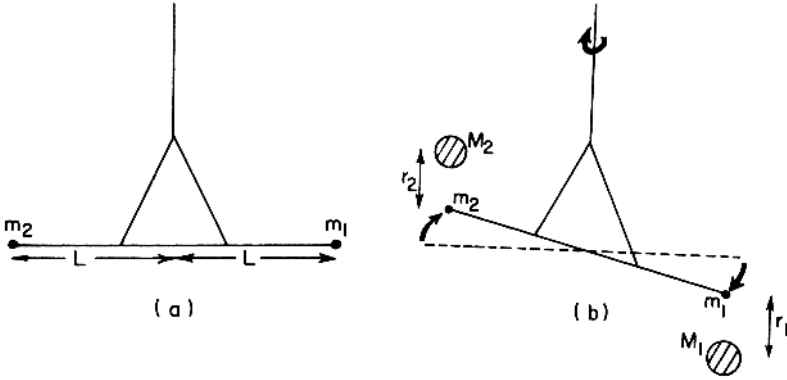
Fig. 3.6. The Cavendish experiment to determine the gravitational constant G .
