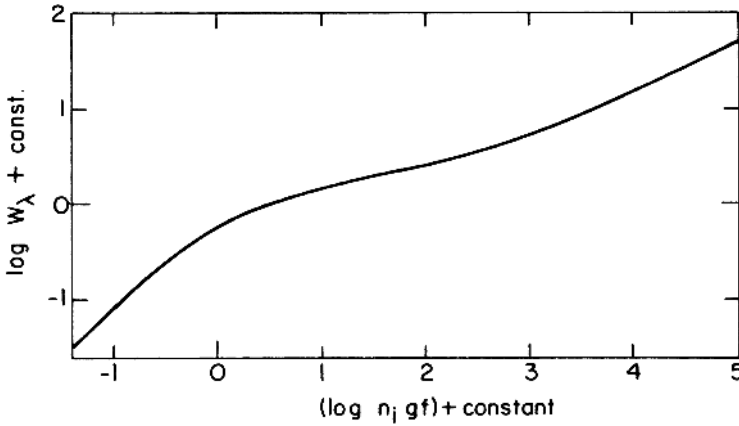
Fig. 7.14. Curve of growth showing increasing absorption with increasing amount of material traversed in a stellar atmosphere. The equivalent width W_\lambda is plotted against n_i g f where n_i is the abundance of an element in a particular energy state, f is the oscillator strength of the Fraunhofer line, and g is the statistical weight of the absorbing state (after A. Unsöld (Un69)).
