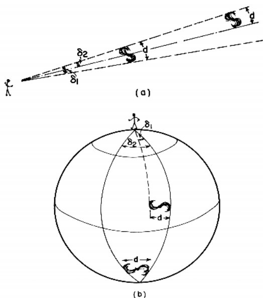
Fig. 11.3. (a) Distance–angular–diameter relation in a flat space. (b) Distance–angular–diameter relation on the surface of a three-sphere.
