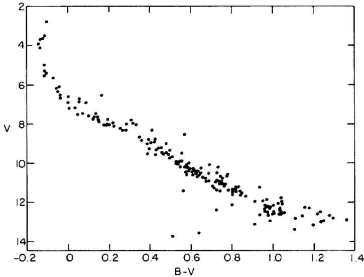
Fig. A.2. Color-magnitude diagram of the Pleiades cluster stars, after correction for interstellar extinction effects. The Pleiades cluster contains some of the most recently formed stars in the Galaxy (after Mitchell and Johnson (Mi57b)).
