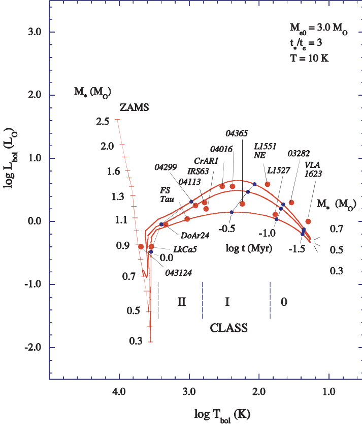
Fig. 1.6. Temperature and bolometric luminosity of protostars. The evolutionary tracks of protostars of 0.3 , 0.5 , and 0.7M_{\odot} are shown proceeding from right to left where the stars reach the zero-age main sequence (ZAMS) and begin consuming their nuclear fuel. A protostar begins life as a Class 0 object, a dense cloud at temperatures in the 8 to 12 K range, glowing at submillimeter wavelengths. Strong bipolar outflows of gas accompany contraction of the central core. Shown here, along with the positions in the H-R diagram of a number of young stellar objects (YSOs), is a set of modeled evolutionary tracks represented by solid lines. The time to fall inward to form a star t_* is taken to be three times the duration of the outflow t_e that dissipates an initially enveloping cloud — t_*/t_e = 3 . The bipolar outflow weakens by the time the protostar evolves to Class I, and abates totally thereafter. A Class 0 object gradually evolves, its temperature rising as it passes through the Class I and II stages before arriving on the ZAMS \sim 30 million years after the onset of contraction. Isochrones — lines of equal age — indicating equal times before arrival on the ZAMS are drawn as straight line segments connecting small dots on the evolutionary tracks. For the tracks shown, the initial mass M_{e0} of the gaseous envelope in which the protostar originally formed has been assumed to be six times the final mass M_{*\infty} of the star. Note the sharp drop in luminosity of these low-mass stars on final approach to the main sequence. In Fig. 1.5, the Hayashi track, shown at the extreme right, corresponds to this drop and shows the same temperature, \sim 4000 K. Courtesy of Philip C. Myers (My98).
