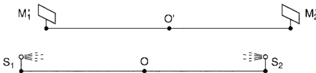
Fig. 5.1. Diagram to describe measurements carried out by observers O and O' in motion at relative velocity V . M'_1 and M'_2 are stationary mirrors equidistant from O'. Sources S_1 and S_2 are equidistant from O and emit flashes of light. S_1 , S_2 , M'_1 , M'_2 , and V all are collinear. O' is moving to the right relative to O.
