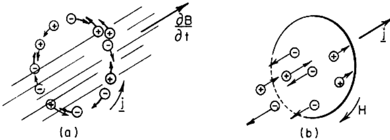
Fig. 6.2. Illustrations for Faraday's and Ampère's laws. (a) Faraday's law states that the current in a conducting loop, and the associated electric field, are determined by the rate of change in the number of magnetic lines of force enclosed by the loop (see equations (6-15) and (6-16)). The number of lines of force crossing unit area is proportional to the magnetic field, \mathbf{B} . (b) Ampère's law states that the magnetic field integrated along a loop enclosing a current is determined by the total current crossing the enclosed area (see equation (6-17)).
