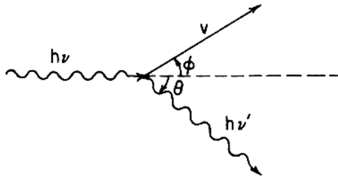
Fig. 6.15. Compton scattering.
