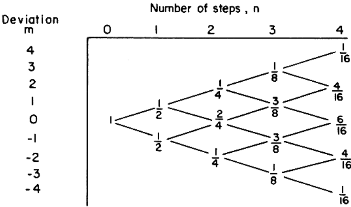
Fig. 4.1. Probability P(m, n) of terminating at position m after n steps.
