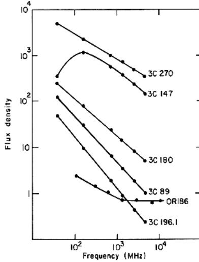
Fig. 6.14. Radio spectra of several extragalactic objects. Note that some have a constant slope, consistent with equation (6-158). Others show considerable curvature. (Compiled from Kellermann, Pauliny-Toth, and Williams (Ke69) and Jauncey, Neill, and Condon (Ja70). Flux density is measured in units of Janskys. 1 \text{ Jy} \equiv 10^{-26} \text{ W m}^{-2} \text{ Hz}^{-1} . With the permission of the University of Chicago Press.)
