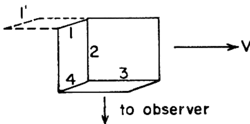
Fig. 5.4. The sides of a rapidly moving cube.
