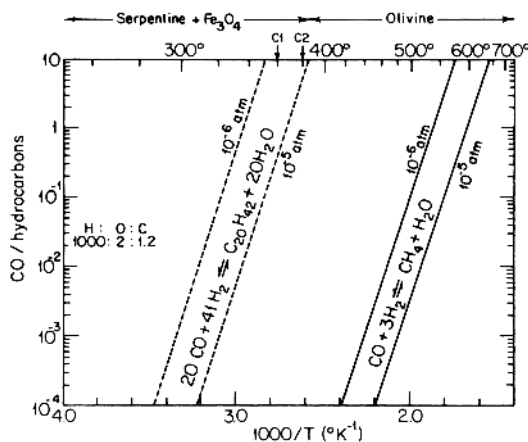
Fig. 10.10. Equilibrium between CO and H 2 at different temperatures and pressures. If equilibrium is maintained on cooling, CO is largely converted into CH 4 before more complex molecules can be formed at lower temperatures. However, this reaction is slow, and some CO may survive to lower temperatures where complex organic molecules can form, particularly if Fe 3 O 4 (iron rust) and hydrated silicates such as serpentine, Mg 3 Si 2 O 5 (OH) 4 , form at 380 to 400 K. Both of these are effective catalysts for the Fischer–Tropsch reaction (see text) (after Anders (An72)).
