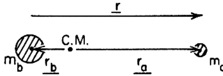
Fig. 3.3. Center of mass (CM) of two bodies a and b . The center of mass of two or more orbiting masses is also referred to as the barycenter .
