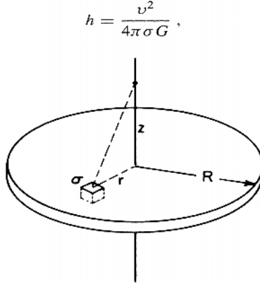
Fig. 9.16. Diagram to illustrate the Galaxy's scale height for stars passing through the plane.
