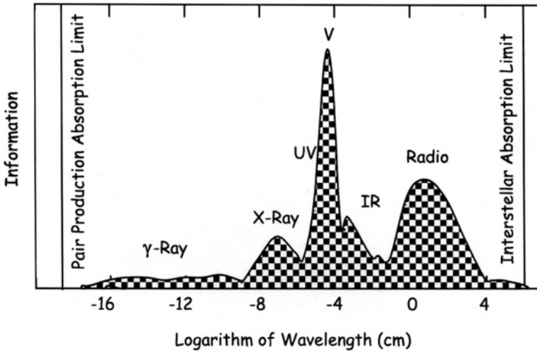
Fig. 1.15. Subjective drawing indicating the amount of information that has been gained through observations in the various portions of the electromagnetic spectrum. The ordinate has a quite arbitrary scale, probably more nearly logarithmic than linear. The peak V represents observations in the visual part of the spectrum.
