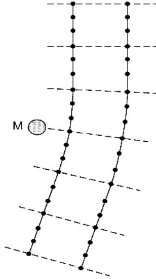
Fig. 5.13. Deflection of light and its wave front due to the gravitational time delay on passage close to a mass M . The wave front, shown by dashed lines, propagates from top to bottom in this figure.
