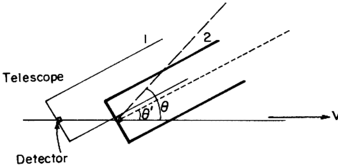
Fig. 5.6. Aberration of light. A telescope (stationary in some coordinate frame K' ) moves with velocity V , relative to a star. When the starlight enters, the telescope is in position 1. By the time the light has traveled the length of the instrument, the telescope has moved to position 2. All this time the telescope is pointed into direction \theta' , with respect to the x' -axis. But an observer whose telescope was at rest with respect to the star's reference frame K would have to point it at angle \theta relative to x . Aberration is also found in Newtonian physics for a finite speed of light c . This is already indicated by the magnitude of the effect, which is of order V/c , whereas purely relativistic corrections are always of order V^2/c^2 and, therefore, are smaller. A relativistic correction needs to be applied to the Newtonian aberration in order to obtain the true aberration angle.
