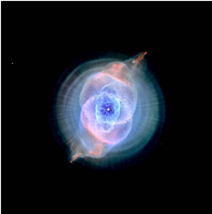
This Hubble Space Telescope image of the Cat's Eye Nebula shows at least eleven shells of gas around the central star, each blown off at a different time.
