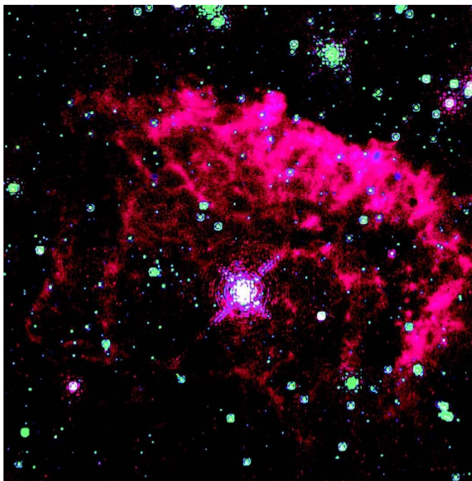
The Pistol Star.
