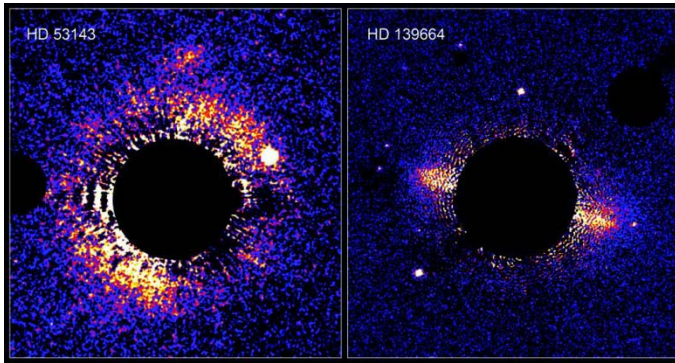
Circumstellar disk around two nearby stars. Data from the Hubble Space Telescope is in false color. Both stars are about 60 light years away. (The black circles are disks used to cut out the glare from the stars.)
