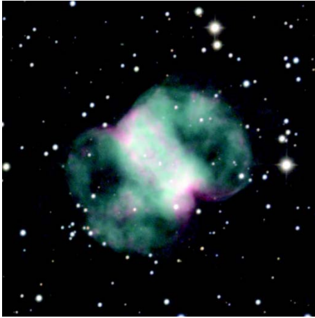
The Little Dumbbell planetary nebula.
