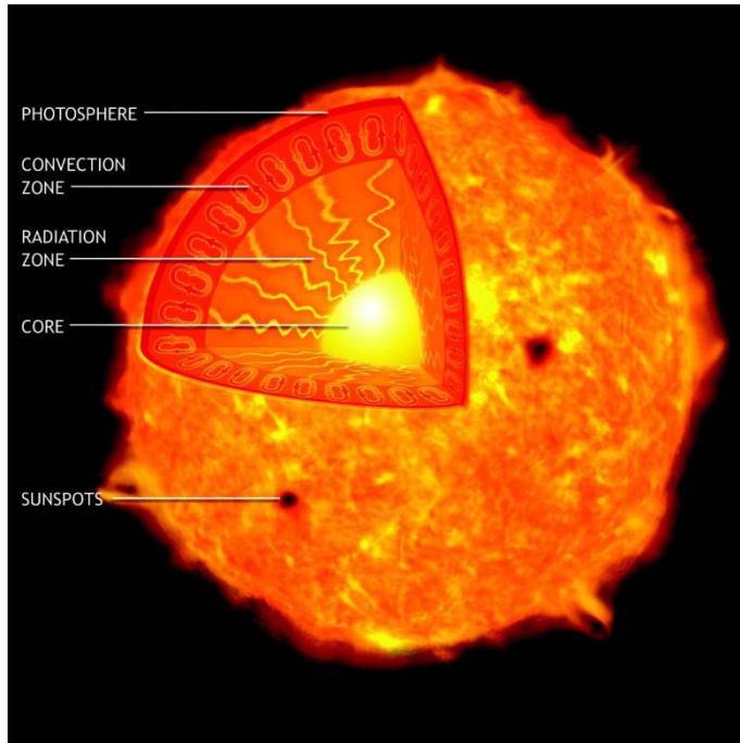
The interior structure of the Sun .
