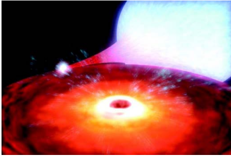
An artist's impression of the accretion disk that forms around a black hole as it draws material from a companion star.
