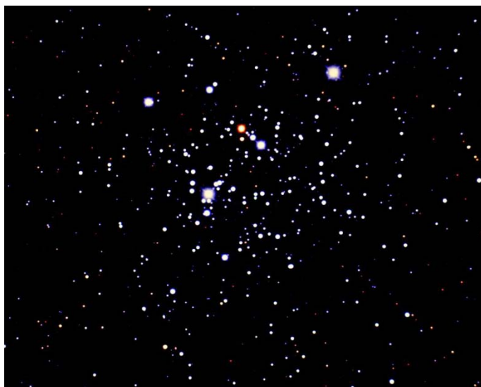
The Jewel Box star cluster.
