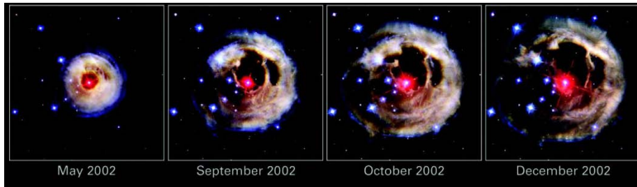
The development of the light echo around a variable star, V838 Monocerotis, following an outburst in 2002.
