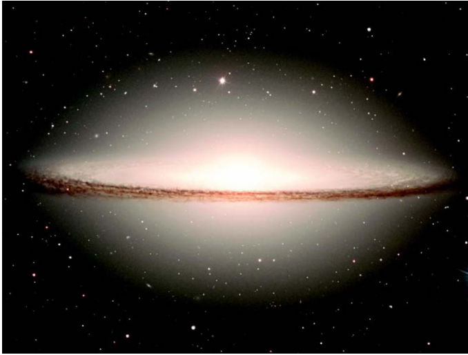
An image of the Sombrero Galaxy from the 8.2-m ANTU unit of the European Southern Observatory's Very Large Telescope.
