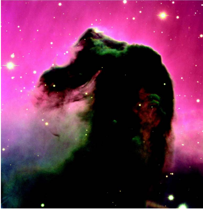
The Horsehead Nebula , imaged by the 8.2-m KUEYEN Telescope of the European Southern Observatory.
