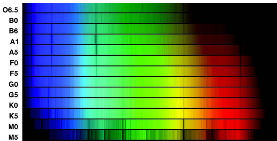
A set of spectra of stars illustrating the range of main spectral types.
