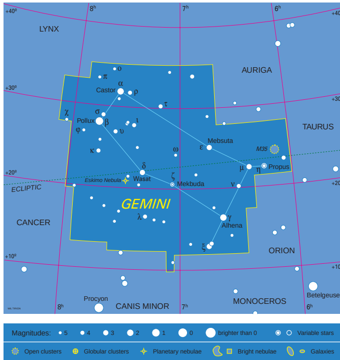
A map of the constellation Gemini .
