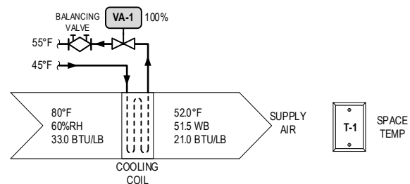
Figure 2 – Cooling Coil with DDC (Single PID)
