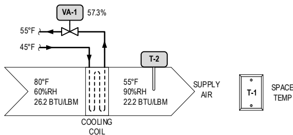
Figure 3 - Cooling Coil with DDC (Cascade Control)
