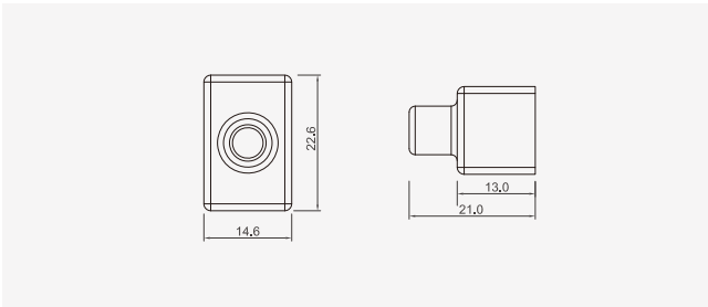
Integral plug
