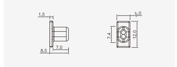
Integral plug
