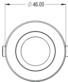
CUT-OUT - 37Ø
