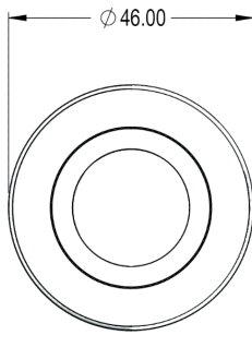
Fixing Screws
