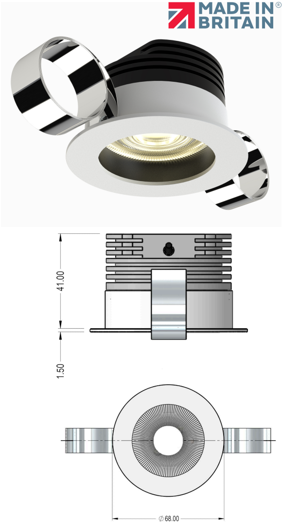
CUT-OUT - 56mmØ
