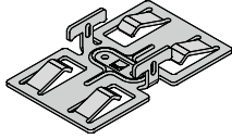
Article 680 Twin-clamp K20* Weight: 45 kg / 1,000 pieces Perforation: 2 x 3.3 mm Ø Material: AlMg3 H22 (EN AW-5754), painted black, RAL 7021
