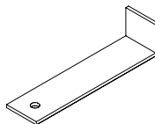
Article 711 Position securing bracket, bright Material: AlMg3 H22 (EN AW-5754) unpainted Box contents: 50 pieces
