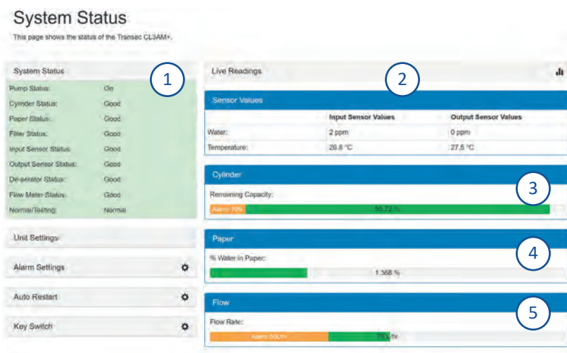
Figure 10. The webserver main screen 1-Alarm Status; 2-Water PPM & Oil Temp from MMT162; 3- Cylinder saturation level; 4-Est. Water content in paper 5-Oil flow rate
