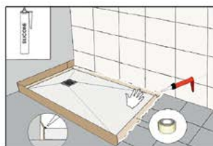
Double sealing with Quare colored silicone
