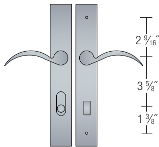
MDLP4 10 1/8" x 1 3/4"
