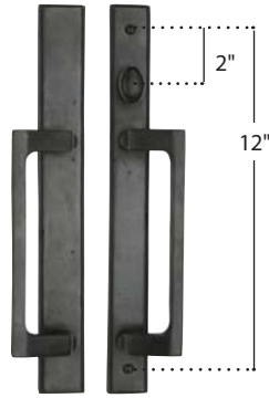
TSL / MTL CONFIGURATION 13 3/4" x 1 1/4" Plate Shown with Dunn Pull
