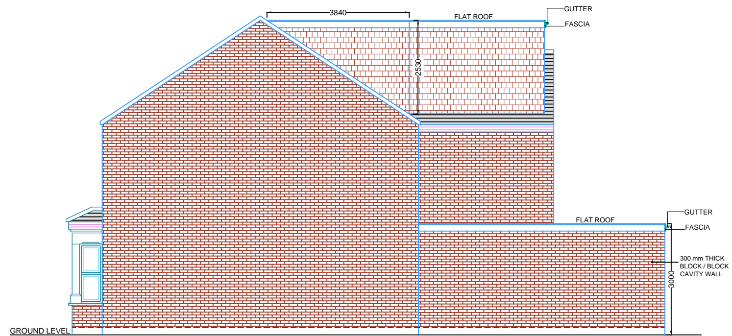
PROPOSED ELEVATION SIDE A
