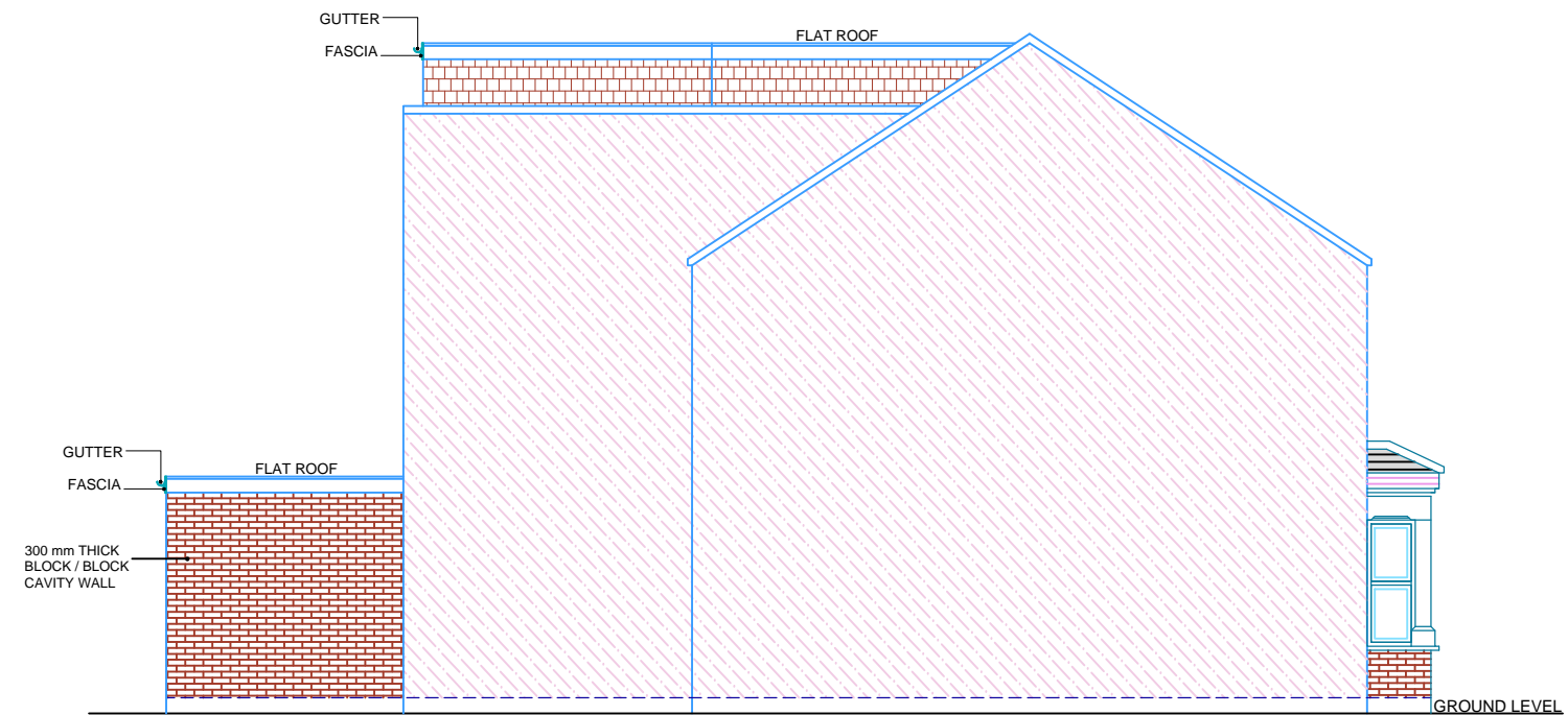
PROPOSED ELEVATION SIDE B
