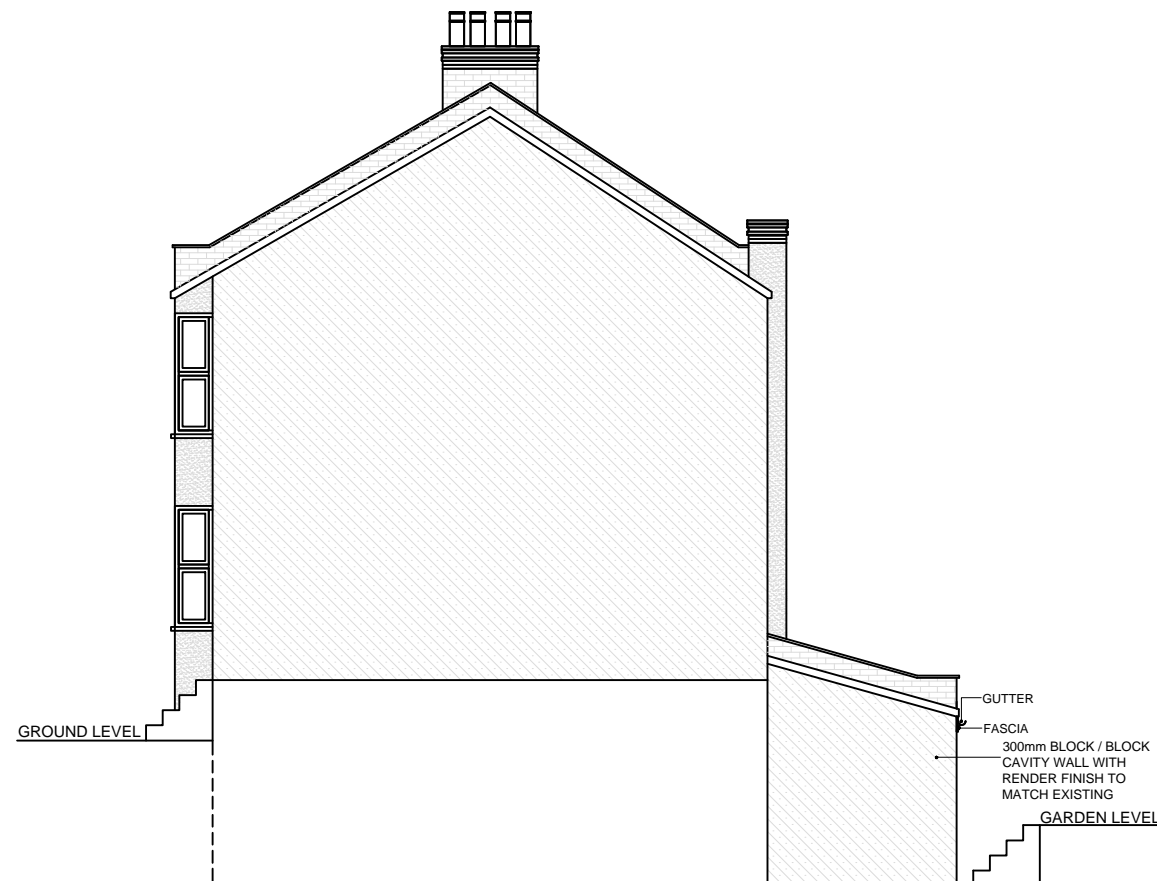
PROPOSED ELEVATION SIDE (A)
