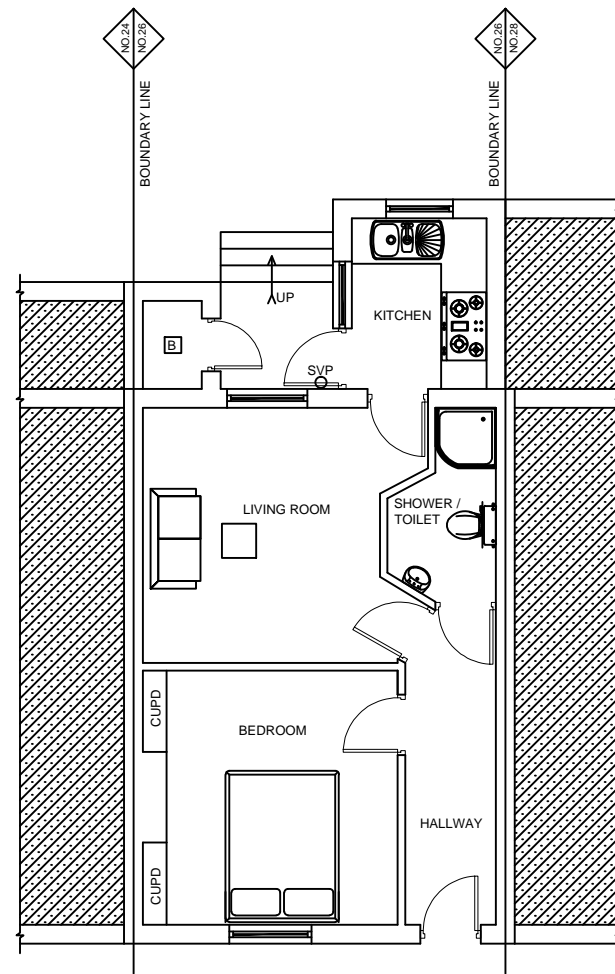
EXISTING LOWER GROUND FLOOR PLAN
