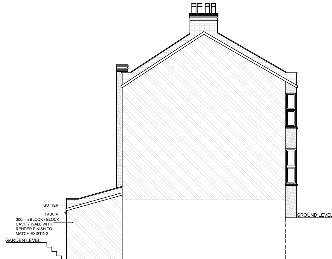
PROPOSED ELEVATION SIDE (B)
