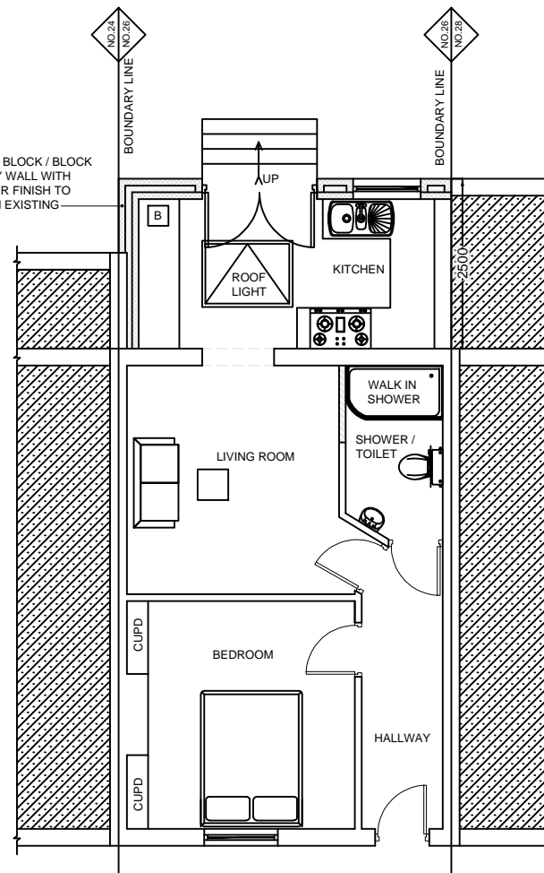
PROPOSED LOWER GROUND FLOOR PLAN
