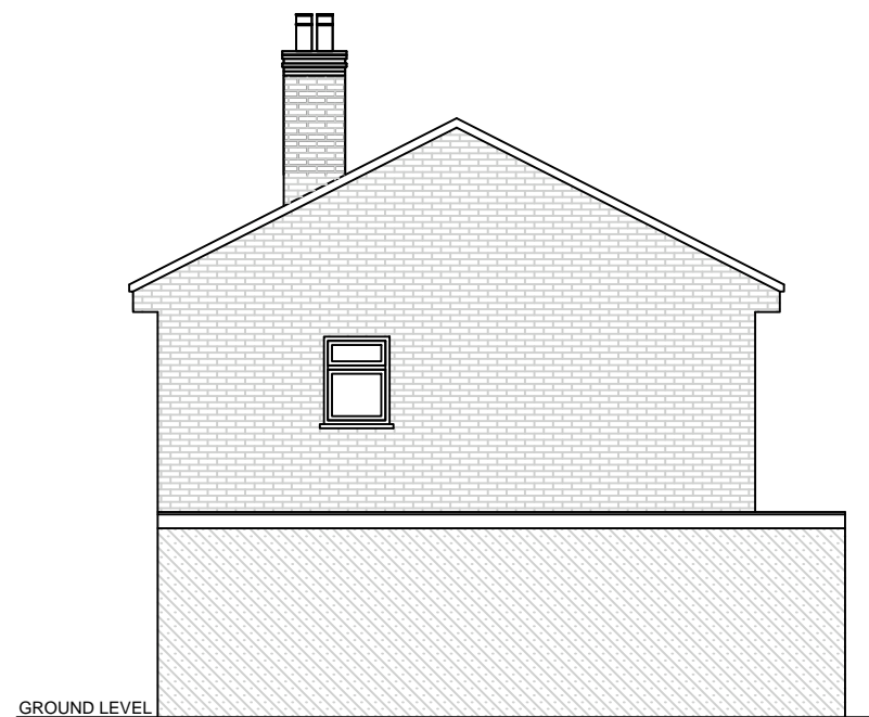
EXISTING ELEVATION SIDE (A)
