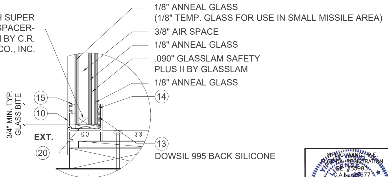
GLASS TYPE "B" 13/16" OVERALL INSULATED LAMINATED GLASS
