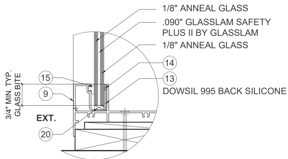
GLASS TYPE "A" 5/16" OVERALL LAMINATED GLASS
