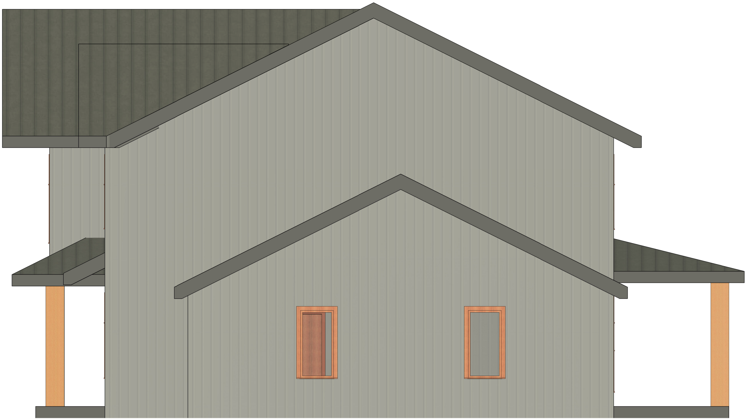
① SIDE ELEVATION 1
