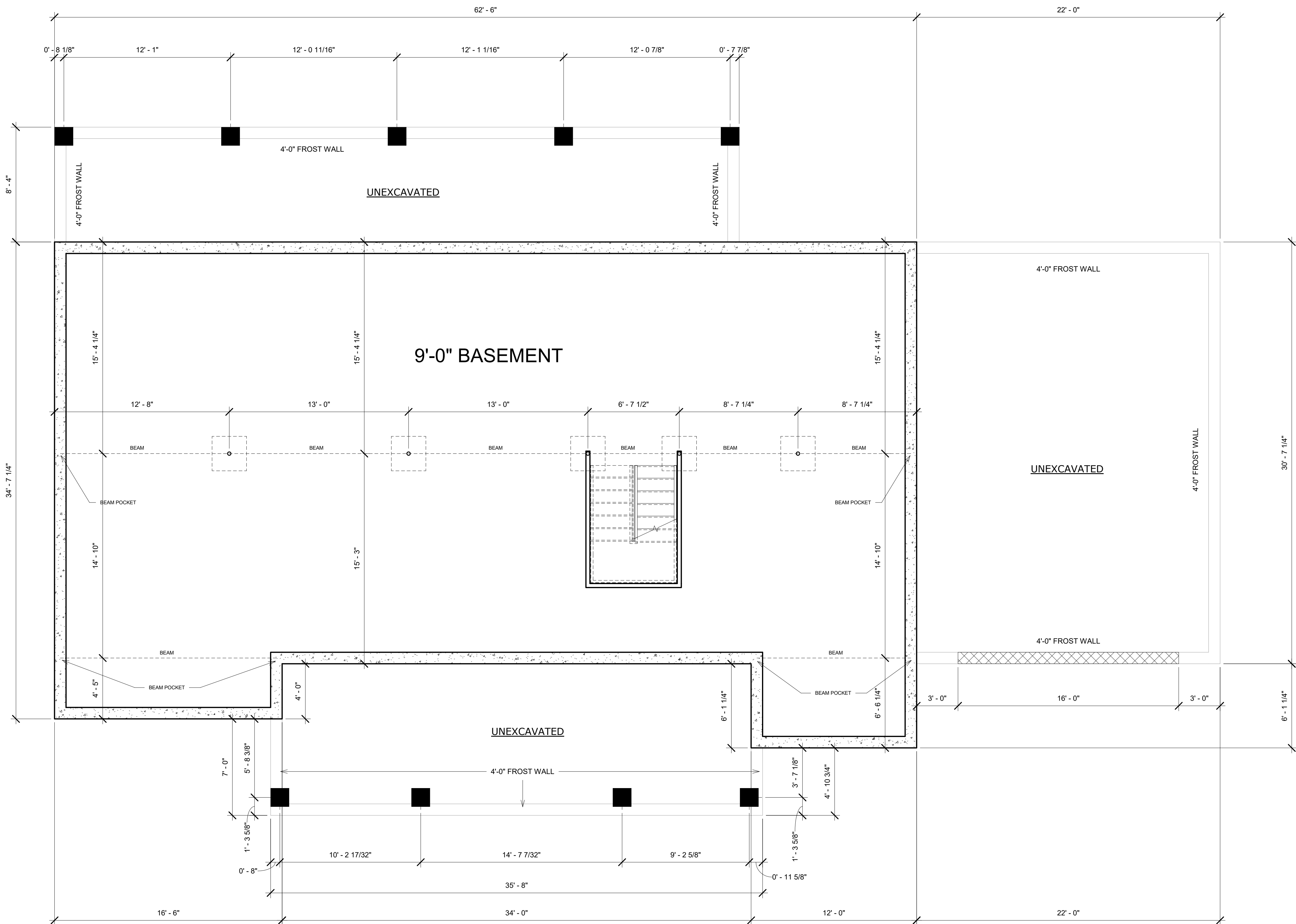
1 Basement 1/4" = 1'-0"
