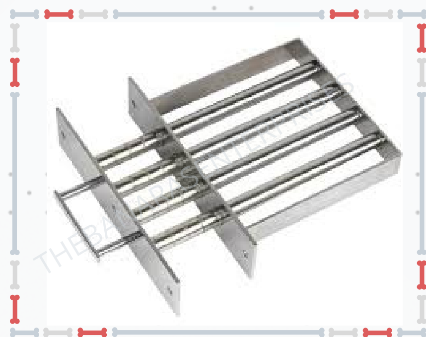
Self Cleaning Magnet
