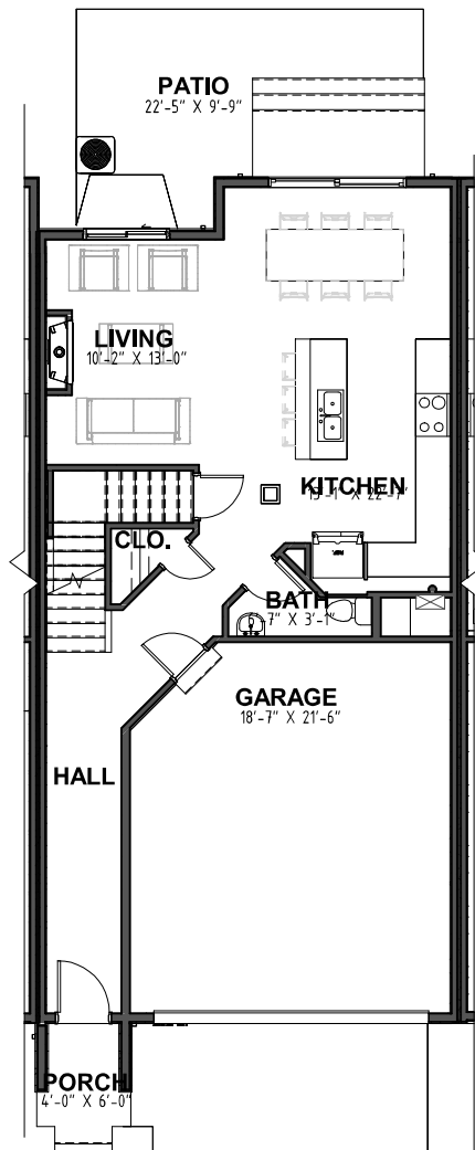
MAIN LEVEL
