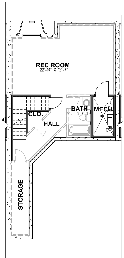
LOWER LEVEL
