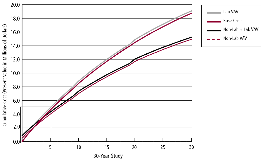
Keck Building Energy Efficiency Retrofit, Life Cycle Cost Analysis – Payback Analysis (in millions of dollars)
