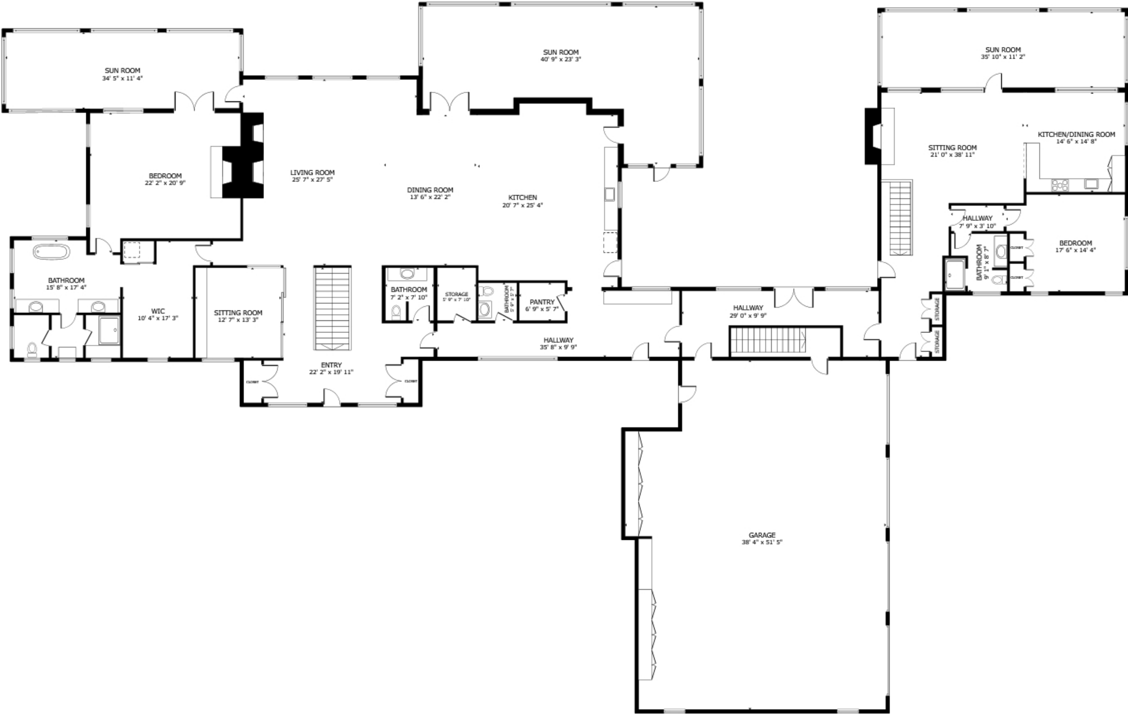
FLOOR 1
