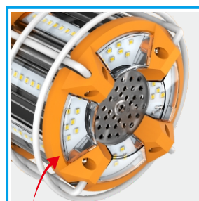
high elasticity PC material to consolidate the bottom of the cage
