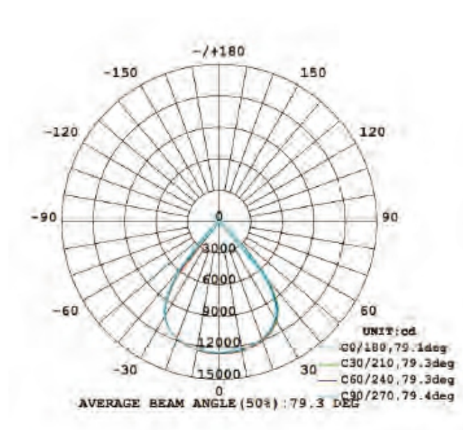
90 Degree
