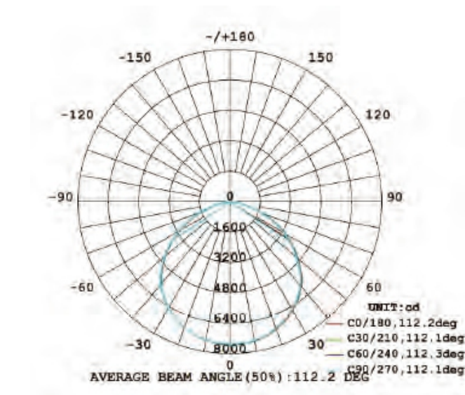
120 Degree
