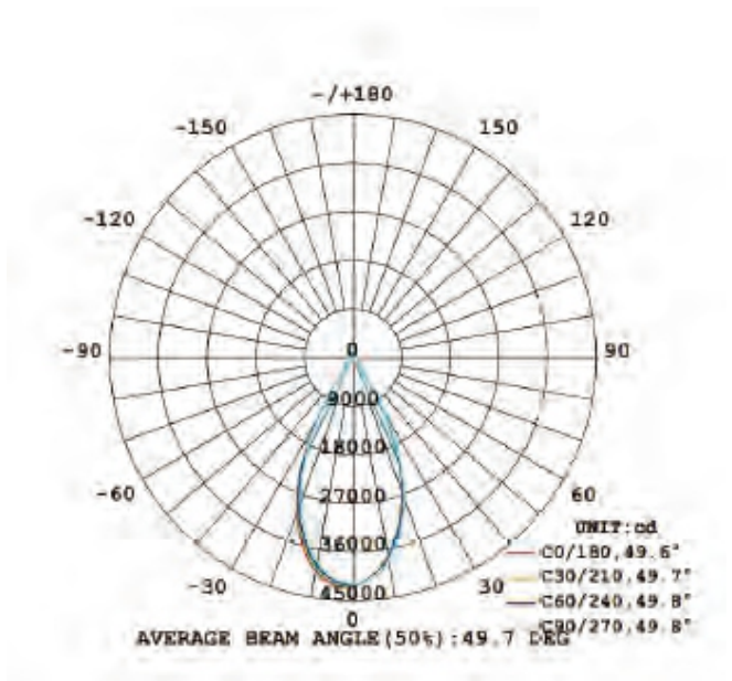
60 degree
