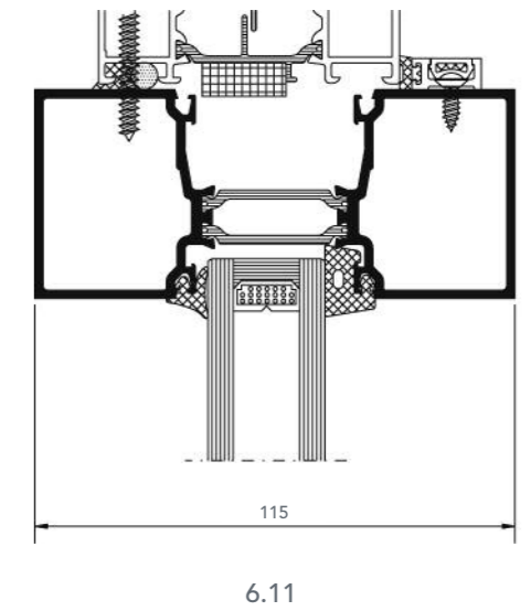
Transom with Window Adaptor (AA®720)
