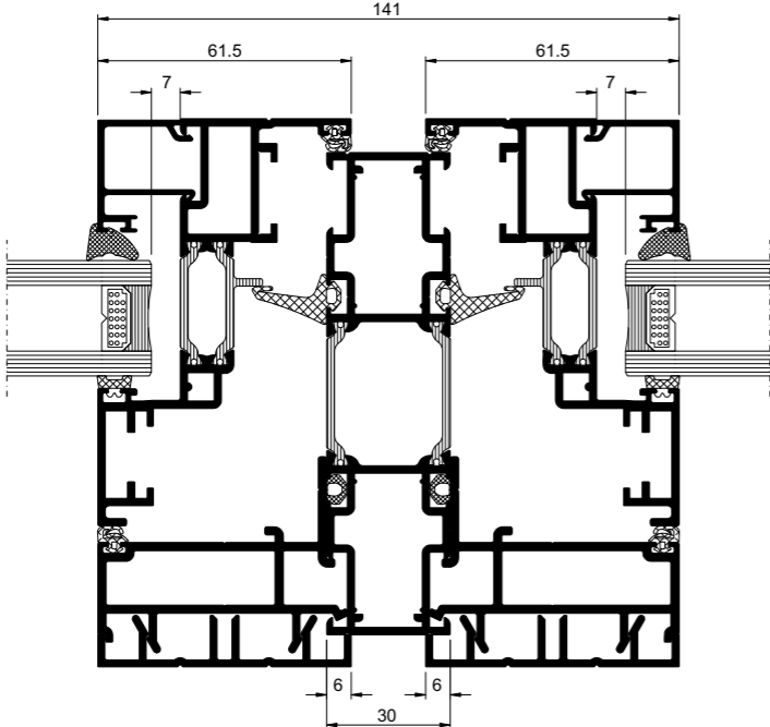
Mullion – Open In Vent/Open In Vent
