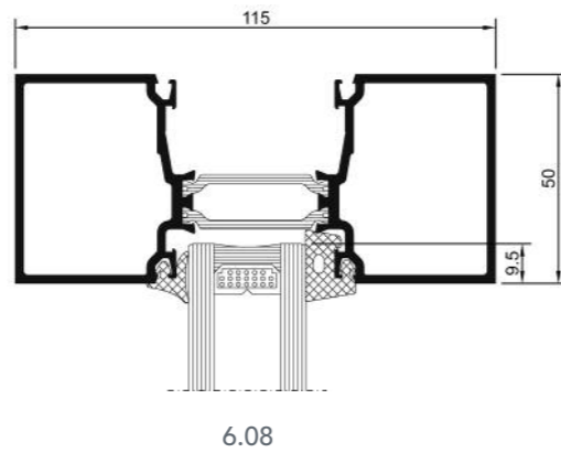
Typical Transom Detail
