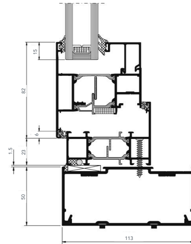
Framing System Door Transom with Opening Vent
