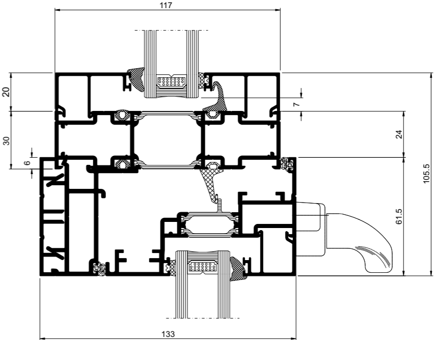
Transom – Fixed Light above Open In Vent
